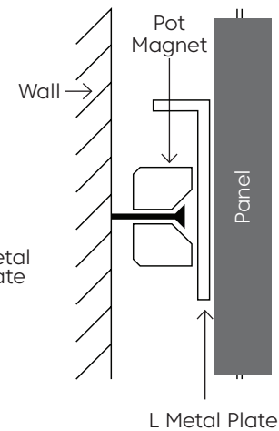
Wall Pot Magnet Install L Plate + Metal Plate
